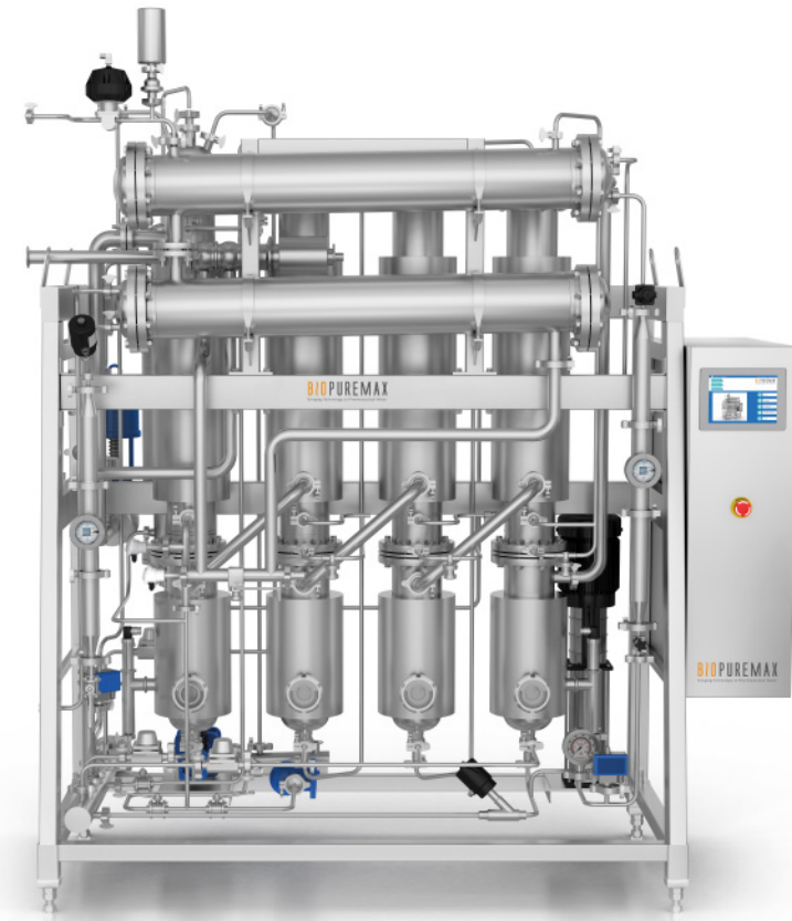
Multieffect Distillation
